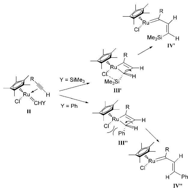
Scheme 2. Stereochemical Aspects of Intermediates III and IV
