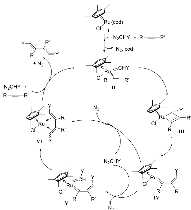
Scheme 1. Proposed Catalytic Cycle
